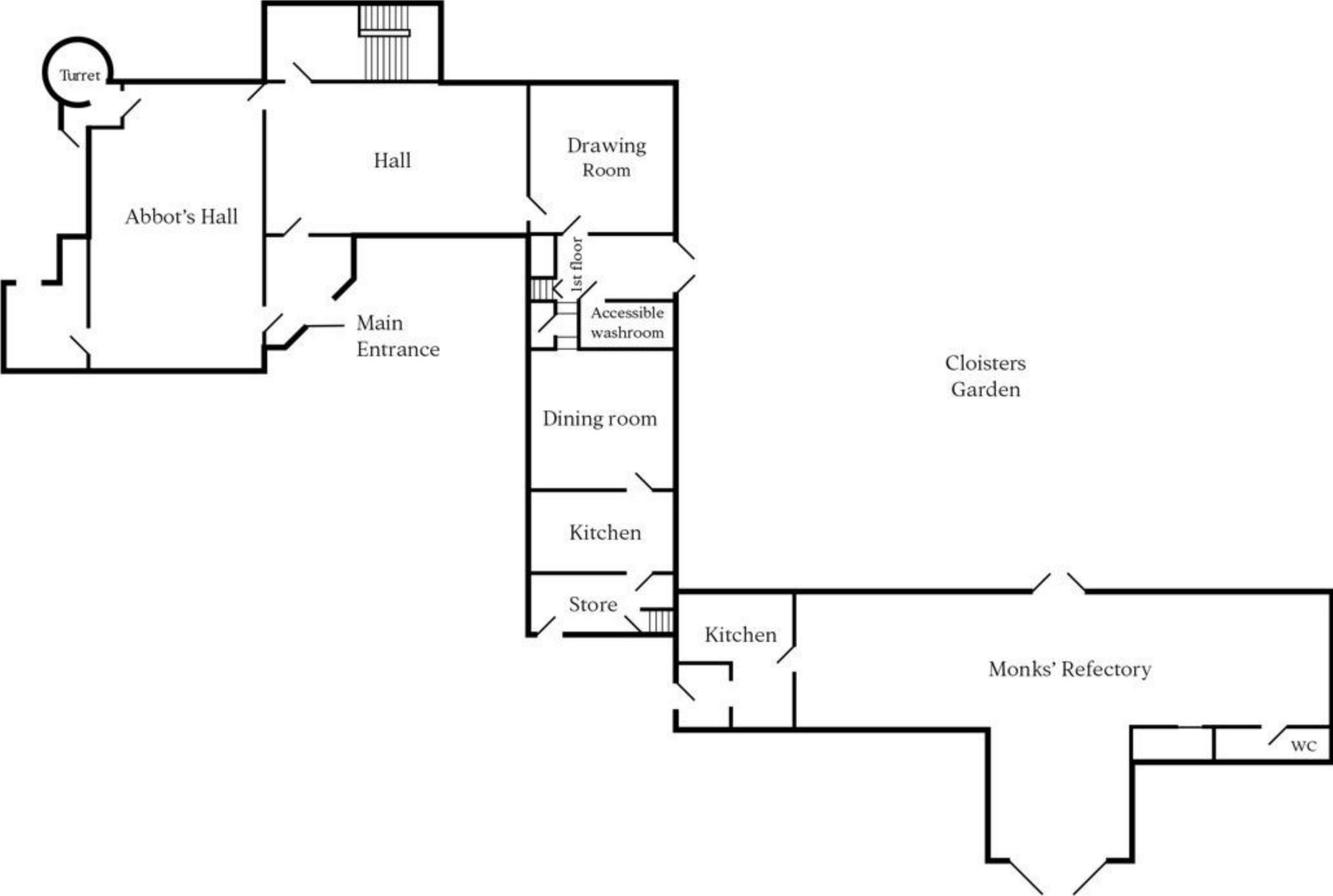
Ground floor
